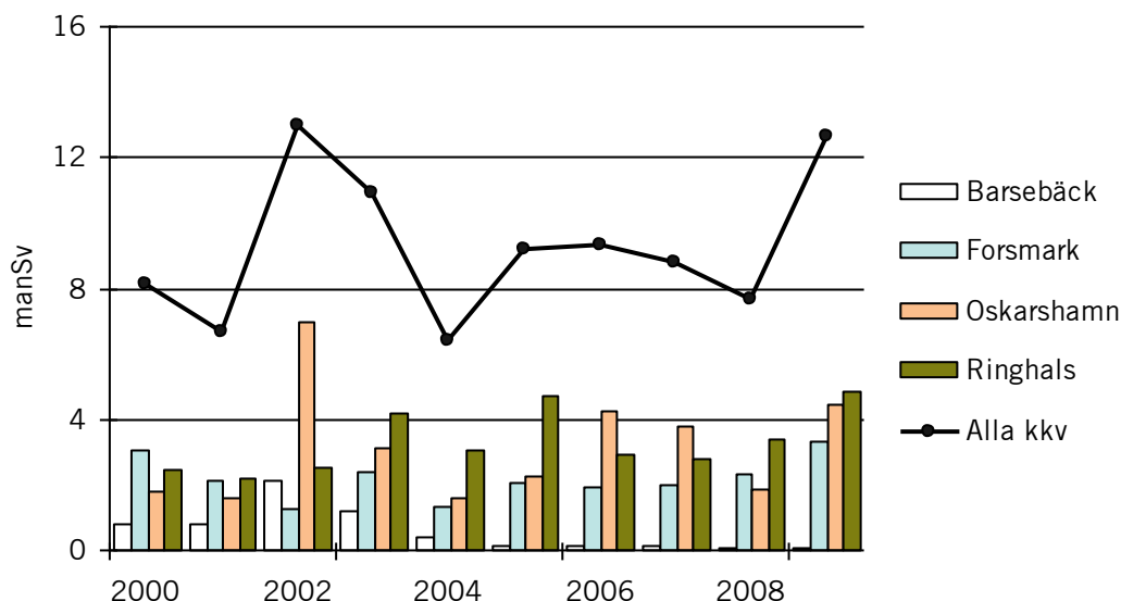
Figure 15. Collective radiation doses at Swedish nuclear power plants during 2000-2009. The radiation levels at the nuclear power plants are stable and variation in collective dose reflects the amount of work and work in “high” radiation areas.
